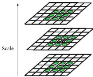
Fig. 4. Process to find the local extrema value
